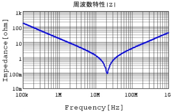
RDER71H103K0K1H03B |Z| DCOV, 25degC
