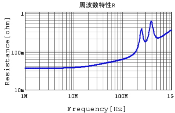
RDE7U2E332J1K1H03B R DC0V, 25degC
