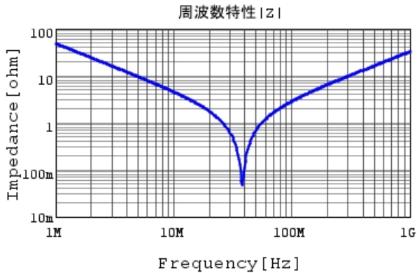
RDE7U2E332J1K1H03B |Z| DC0V, 25degC
