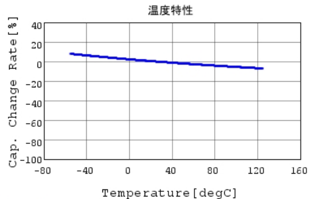
RDE7U2E332J1K1H03B C-Temp. capchange, DC0V,
