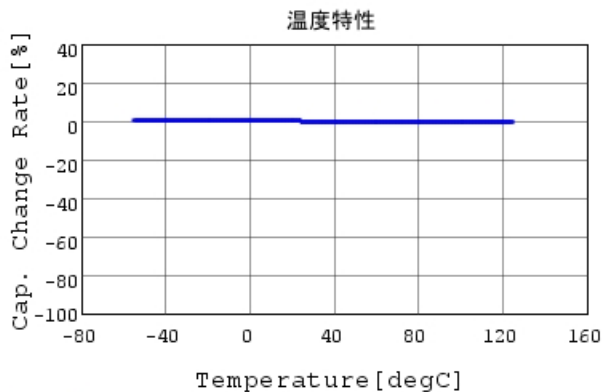
RDE5C1H102J0K1H03B C-Temp. capchange, DC0V,
