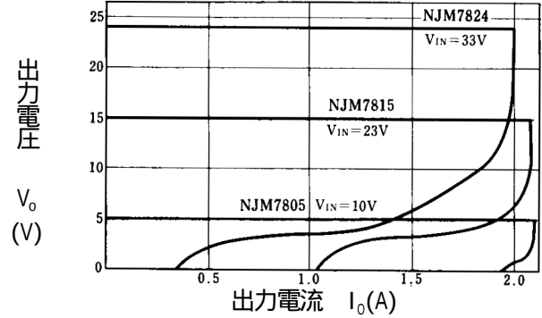
NJM7805/15/24 負荷特性例 ( T_j = 25 )
