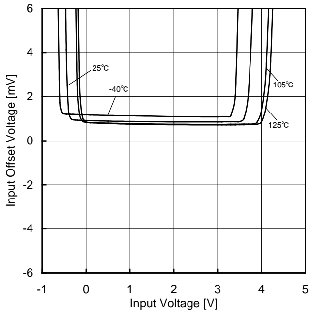
Figure 105. 同相入力電圧範囲 (VCC=5V)
