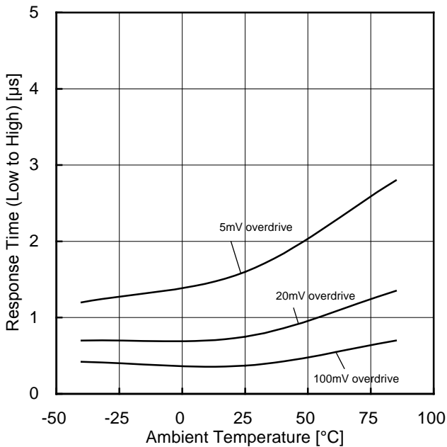
Figure 63. L→H 応答時間-温度特性 (VCC=5V, VRL=5V, RL=5.1kΩ)
