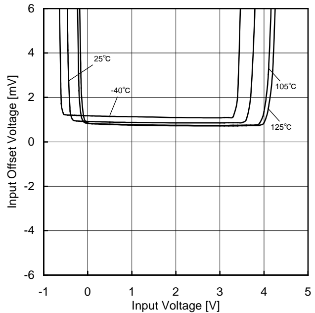
Figure 82. 同相入力電圧範囲 (VCC=5V)
