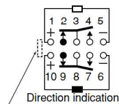
• 2-coil latching (Reset condition)
