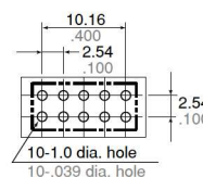
PC board pattern (Copper-side view)
