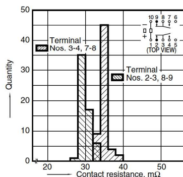
10. Distribution of contact resistance Tested sample: TQ2SA-5V, 30 pcs. (30 \times 4 contacts)
