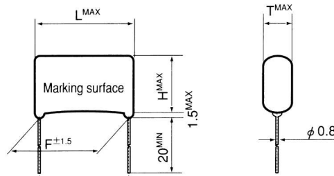
Drawings and dimensions
