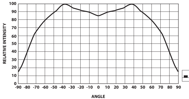
Figure 6. Relative intensity vs. angle for HSMx-C120.
