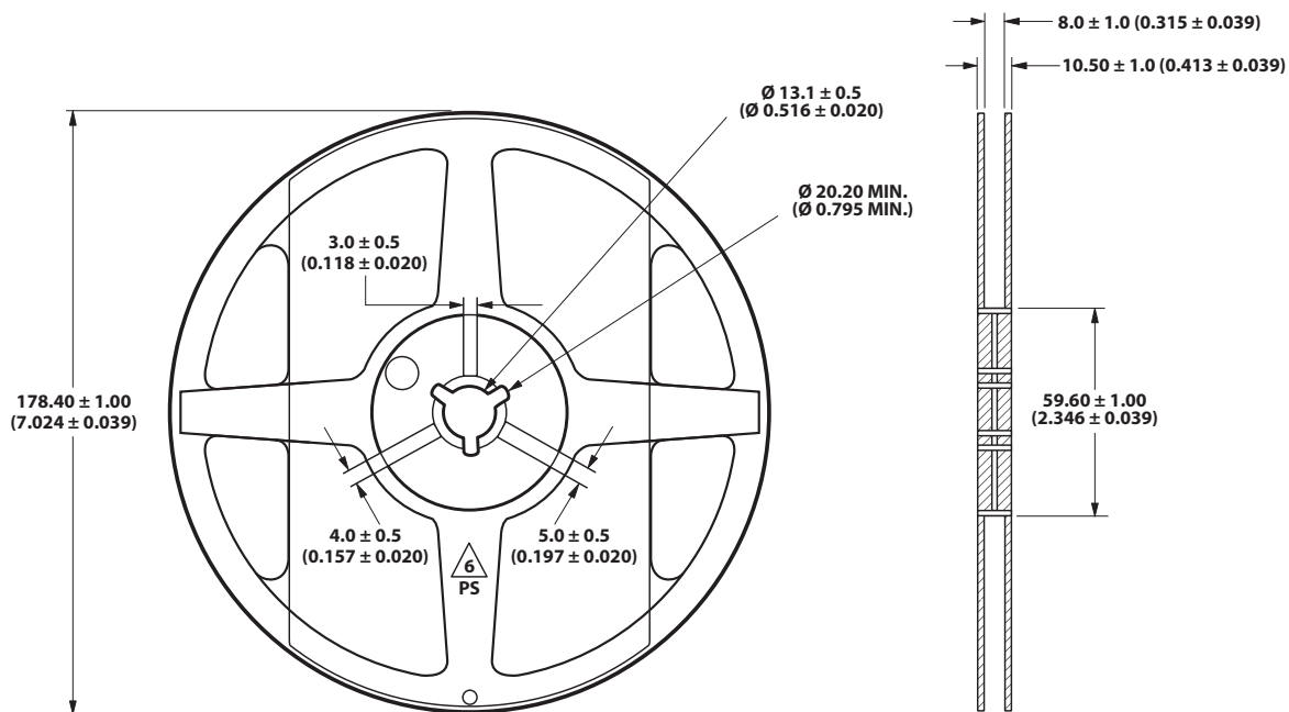
Figure 18. Reel dimensions.
