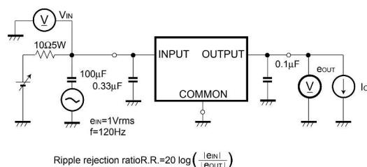
Fig. 2 Measurement circuit for ripple rejection ratio
