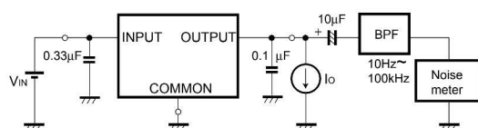
Fig. 3 Measurement circuit for output noise voltage
