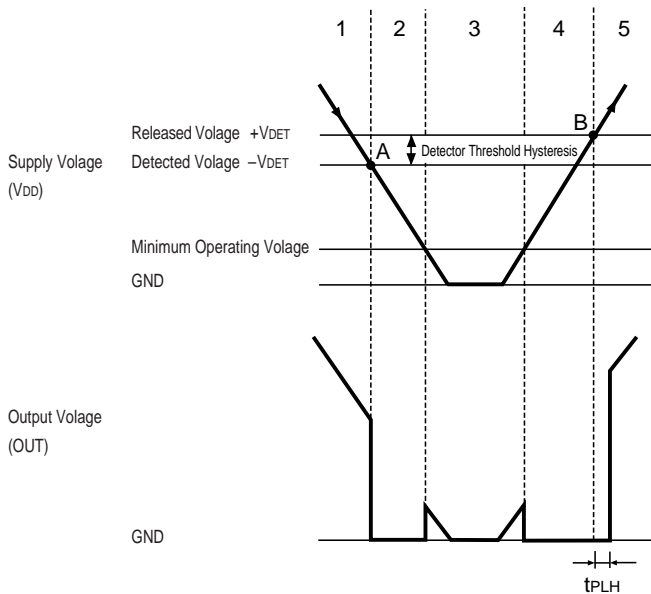
FIG. 2 Operation Diagram
