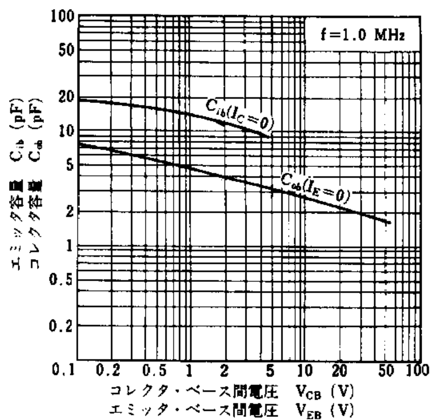
INPUT AND OUTPUT CAPACITANCE vs. REVERSE VOLTAGE
