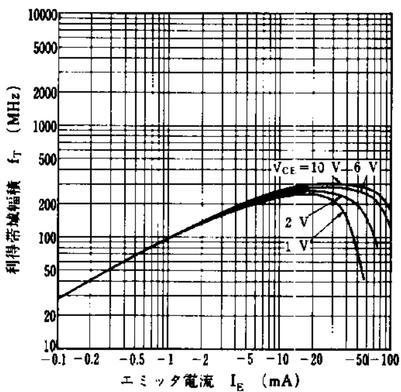
GAIN BANDWIDTH PRODUCT vs. EMITTER CURRENT
