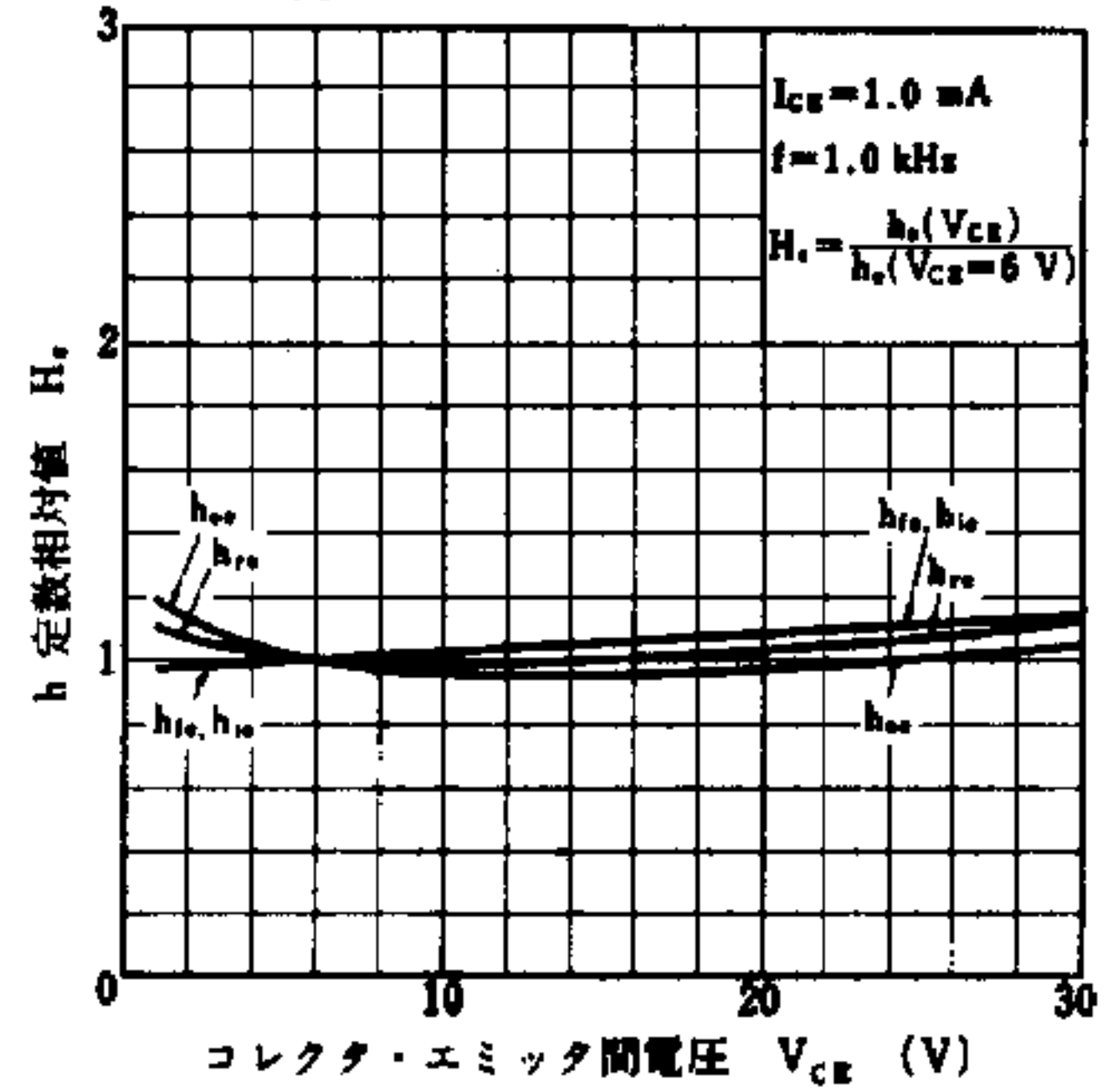
NORMALIZED h-PARAMETER vs. COLLECTOR TO EMITTER VOLTAGE
