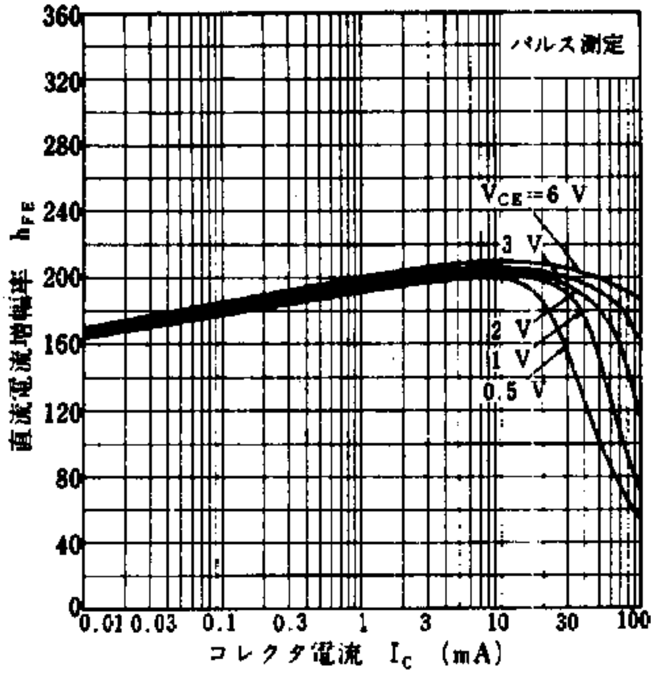
DC CURRENT GAIN vs. COLLECTOR CURRENT
