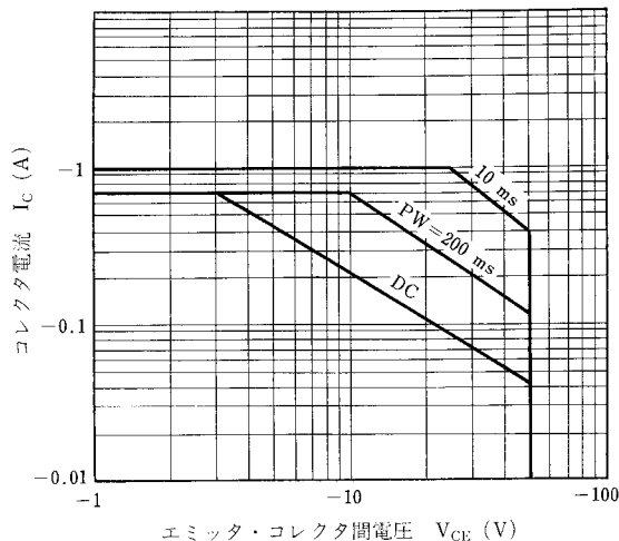
SAFE OPERATING AREA (TRANSIENT THERMAL RESISTANCE METHOD)
