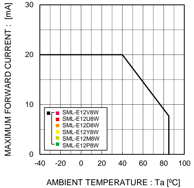
Fig.6 Derating
