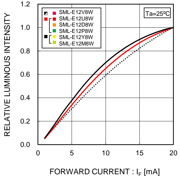
Fig.4 Luminous Intensity - Forward Current
