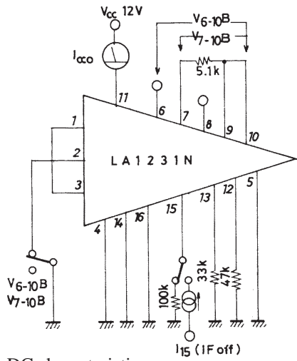
DC characteristics
