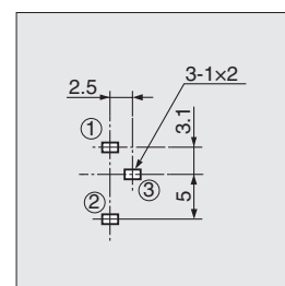
Hole Layout (Bottom View)
