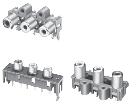
3連／Triple Type
